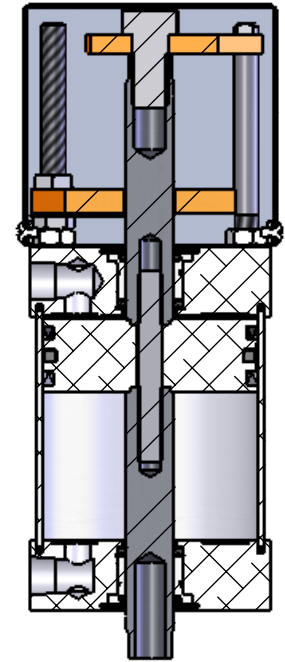
SECTION Z-Z SCALE 1 : 4
