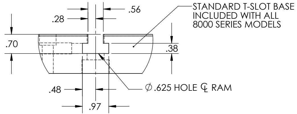
DETAIL X SCALE 1 : 2
