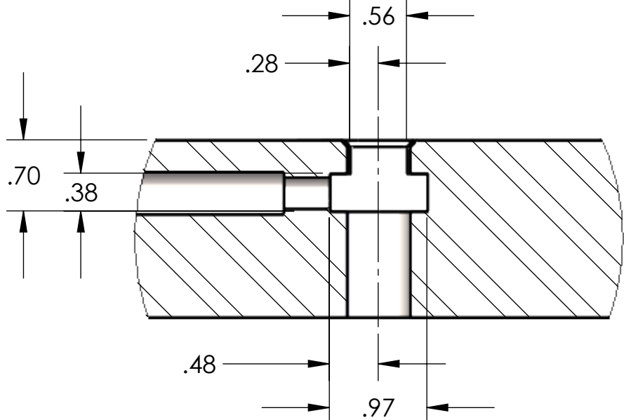
DETAIL D SCALE 3 : 4
