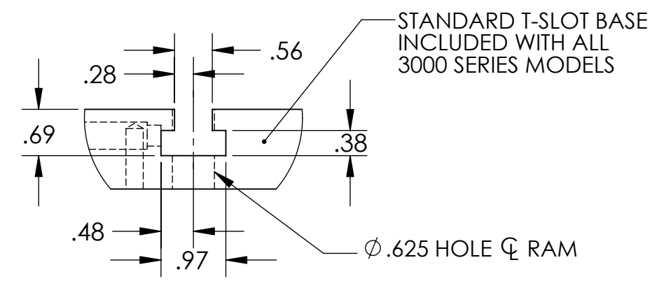
DETAIL X SCALE 1 : 2
