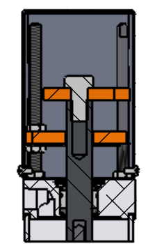
SECTION Z-Z SCALE 1 : 4
