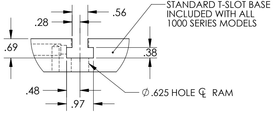
DETAIL X SCALE 1 : 2
