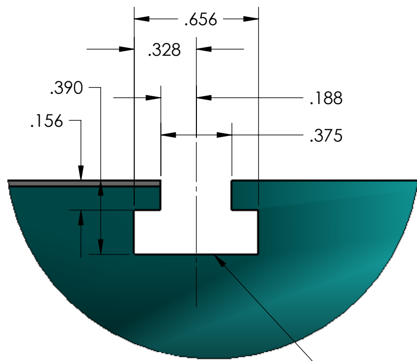
DETAIL A SCALE 2 : 1 SLOT FOR 5/16 T-BOLT
